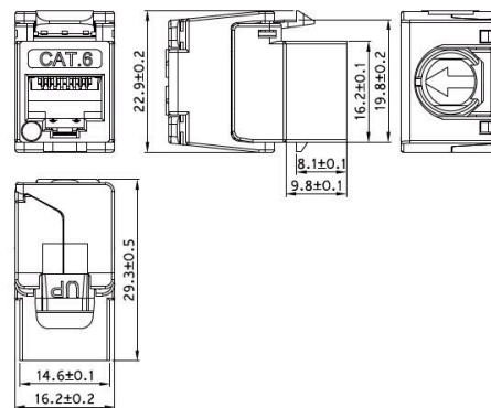
Schematics drawings
